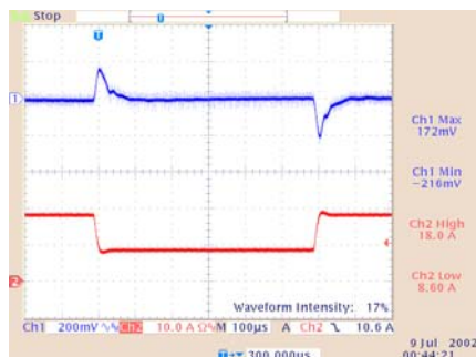
Transient response of UQ48050abcd-50XXX ( V_{IN} : 50V, Load: 18.0A/8.5A@2.5A/μs)
