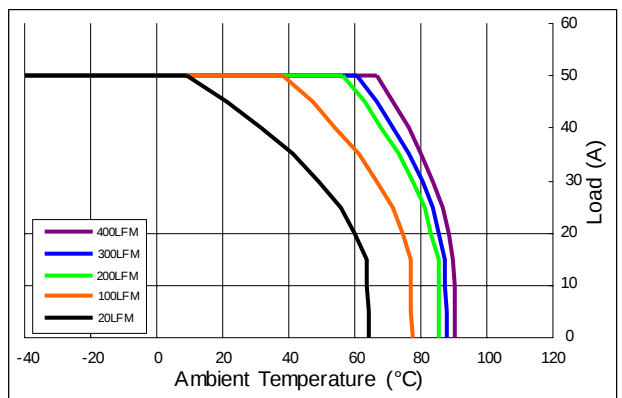
Derating curves of UQ48050abcB-50XXX for T_C = 110°C
