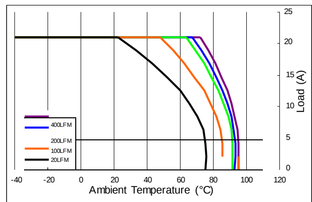
Derating curves of UQ48120abcB-21XXX for T_C = 110°C
