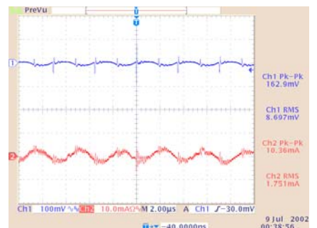
Input/Output ripples of UQ48050abcd-50XXX ( V_{IN} : 50V, Load: 50A, L_{IN} =10uH)
