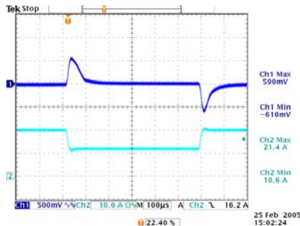
Transient response of UQ48120abcd-21XXX ( V_{IN} : 50V, Load: 21.0A/10.5A@2.5A/μs)
