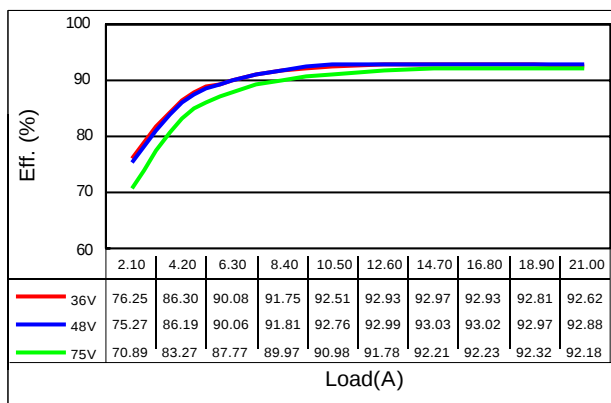
Efficiency plot of UQ48120abcB-21XXX
