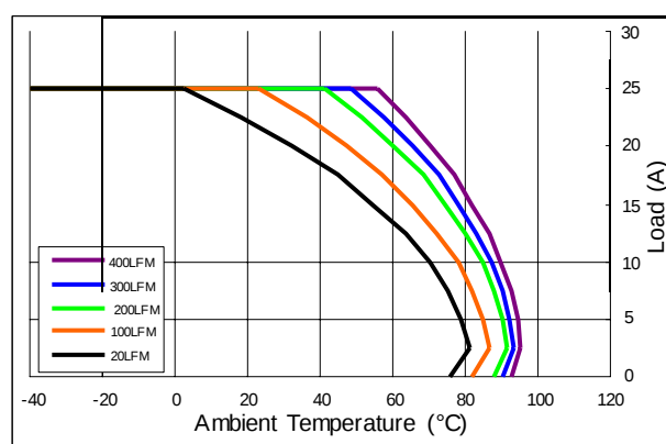
Derating curves of COE48050abcA-25XXX for T_c = 110^\circ\text{C}
