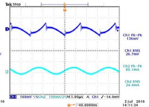
Input/Output ripples of CPH48050abcd-70XXX ( V_{IN} : 48V, Load: 70A, L_{IN} =10μH)
