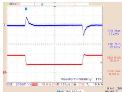
Transient response of CPH48033abcd-70XXX ( V_{IN} : 48V, Load: 18A/8A@2.5A/μs)
