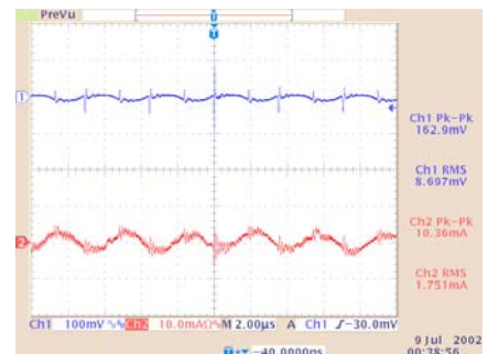
Input/Output ripples of CPH48033abcd-70XXX ( V_{IN} : 48V, Load: 70A, L_{IN} =10μH)
