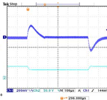
Transient response of CPH48050abcd-70XXX ( V_{IN} : 48V, Load: 52.5A/35.0A@2.5A/μs)
