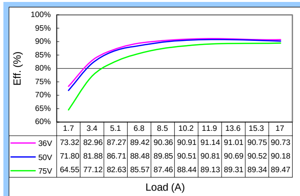
Efficiency Plot of CPH48150ABCD-17
