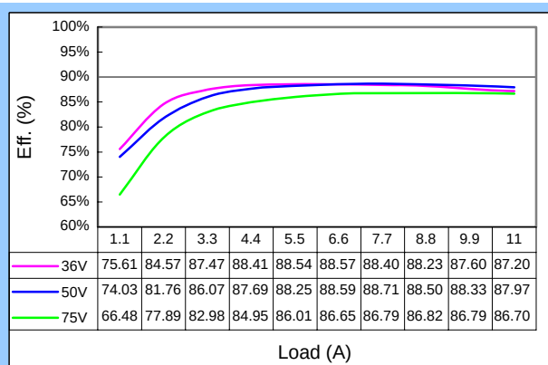
Efficiency Plot of CPH48240ABCD-11
