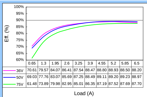
Efficiency Plot of TSH48240ABCD-07
